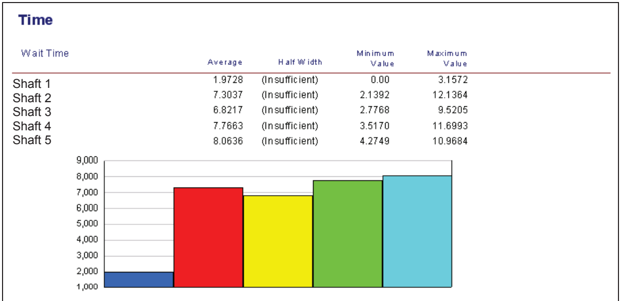
Fig.17. The example of results from simulation – average waiting time for different shafts
